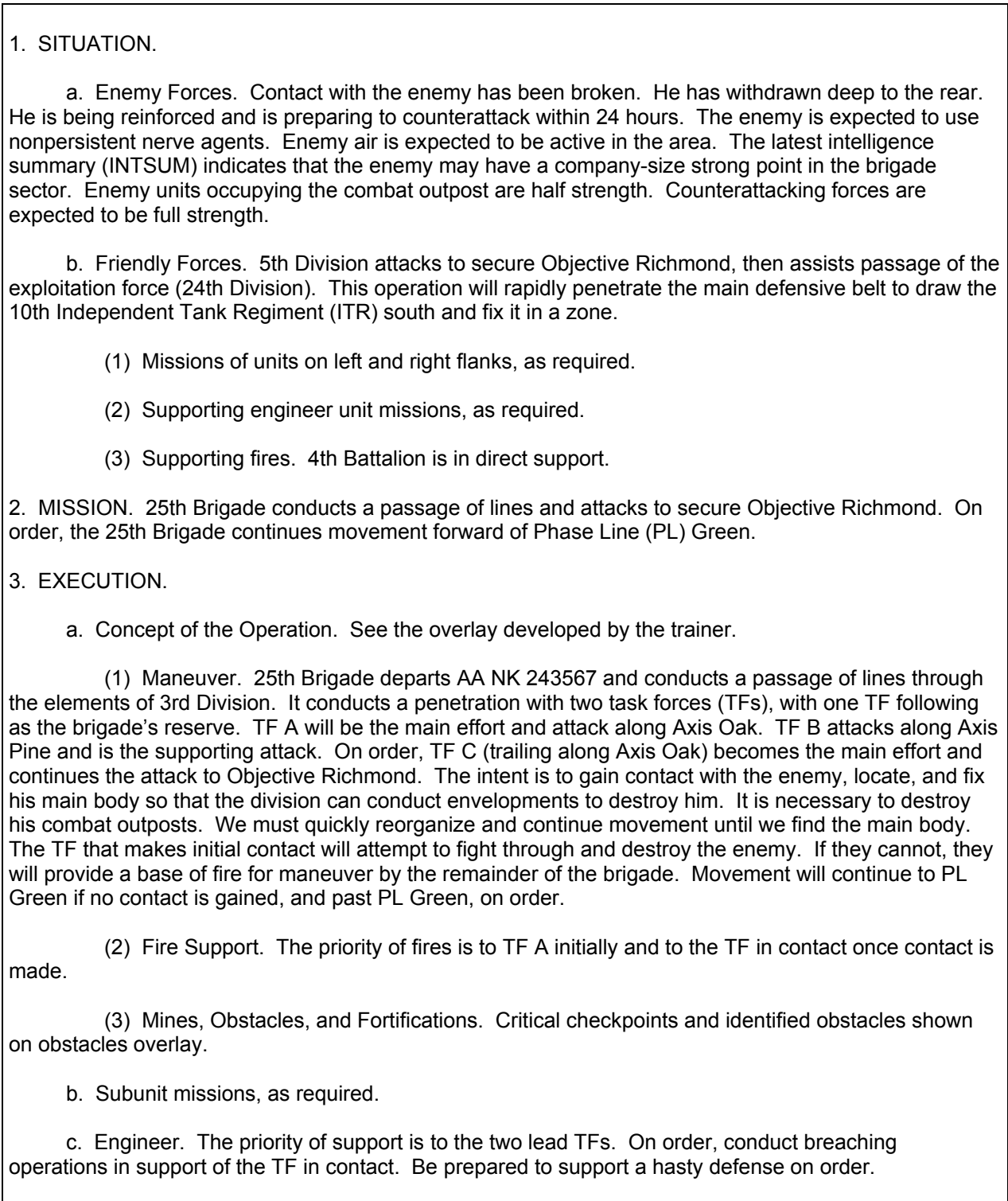
Figure 4-3. Sample OPORD
